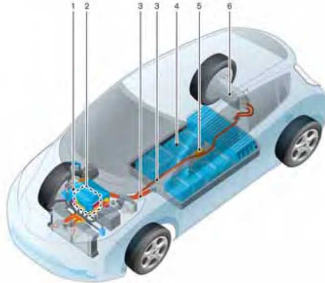
High-voltage components
