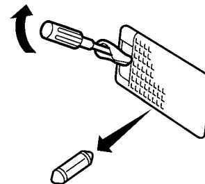
Cargo light
