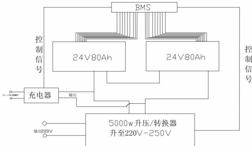
7-5 工作原理图 Working principle diagram
