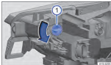
Fig. 159 Rear of the right headlight: changing the turn signal bulb.
