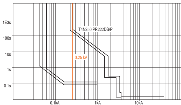
T4N 250 PR222DS/P-LSIG In 250 A
