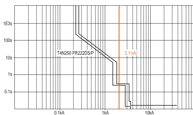
T4N 250 PR222DS/P-LSI In 250 A
